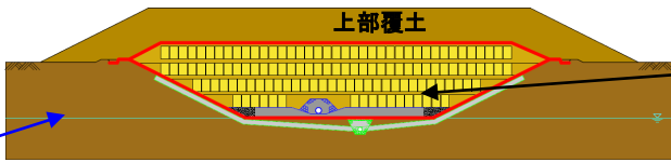
トレンチ埋設施設 (付加機能型) Trench with prevention system from permeation and leakage of water
