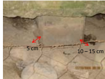
Pile foundation of bridge
